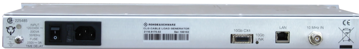
Figure 1-2 CLG Rear Panel
